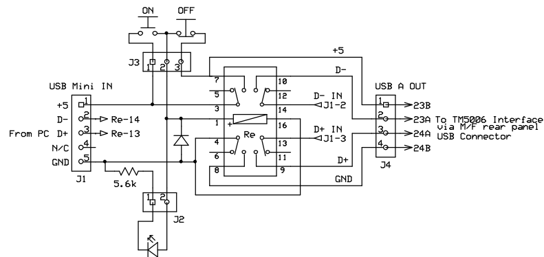
External Switch to manually enable Rear USB only when needed
